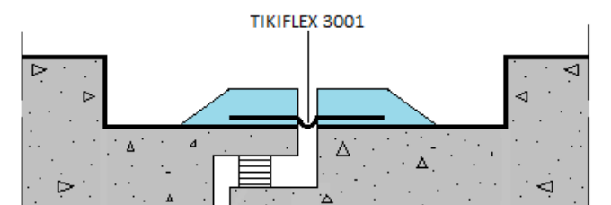
Waterproofing of Specific Joints
